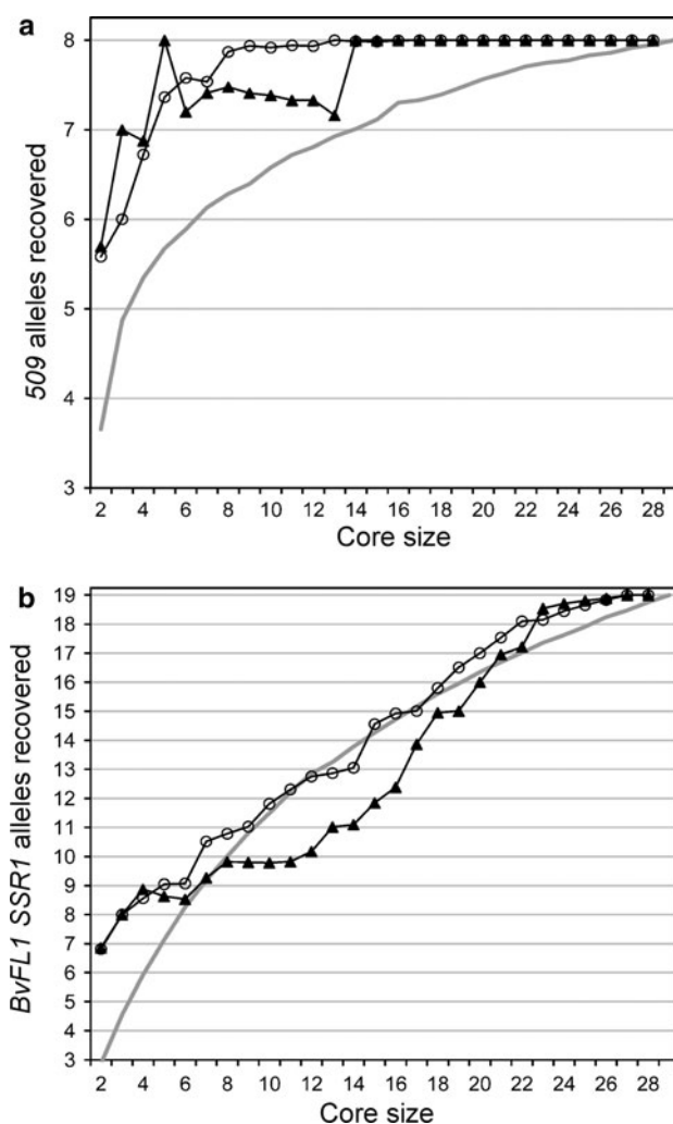
Fig. 3 Effect of core subset optimization algorithms on recovery of allelic diversity at neutral and selected target loci in Beta vulgaris ssp. maritima . Number of alleles retained in the core using random selection indicated with smooth gray line. Allelic retention using standard MSTRAT algorithm (M) shown with solid triangles. Improved algorithm (M+) shown with open circles. Both optimization algorithms performed well when targeting (a) neutral locus 509, but failed when targeting (b) selected locus BvFL1 SSR1 . M+ outperformed M in both cases
